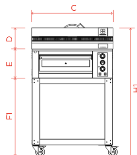
Front view / Pyralys HP 4
