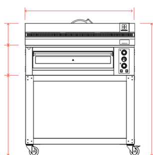
Front view / Pyralys HP 6L
